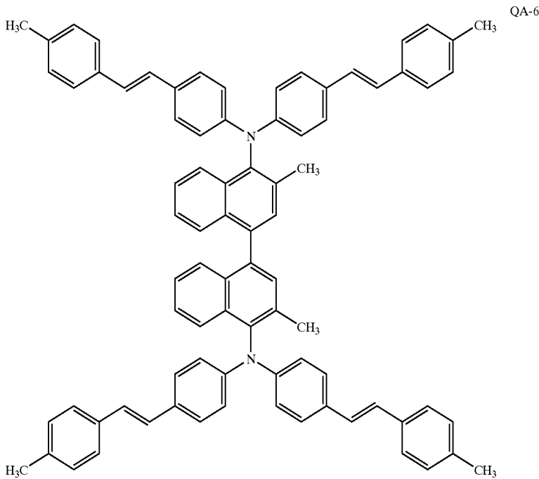
Compound described in JP-A 11-152253
