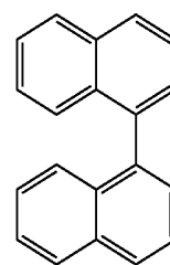
1, 1'-binaphthyl
