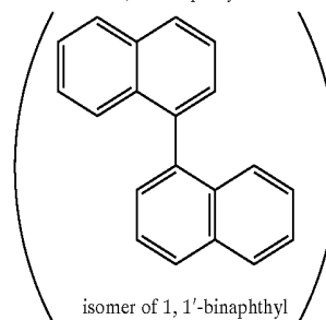
1, 1'-binaphthyl
